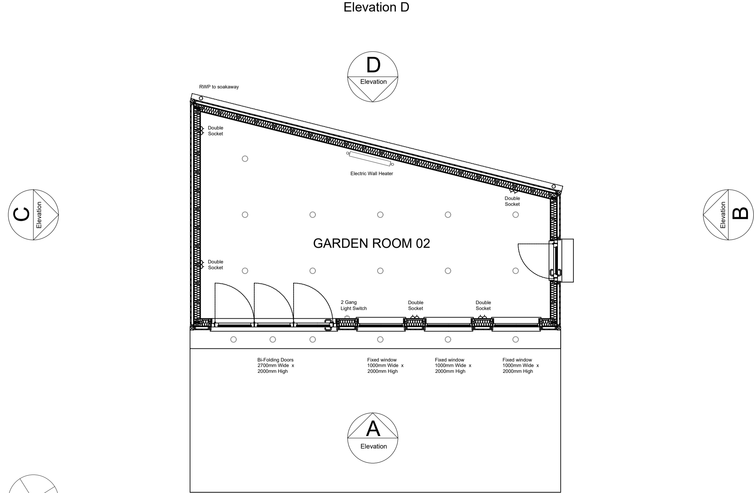
Proposed Plan and Elevations 1:50 @ A1
