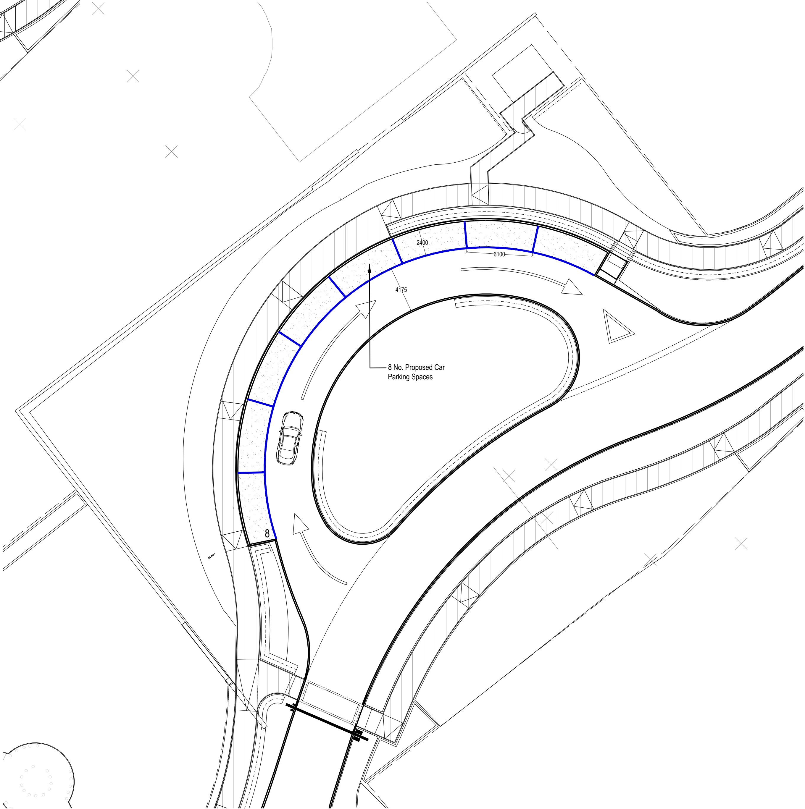
Proposed Car Parking Layout
