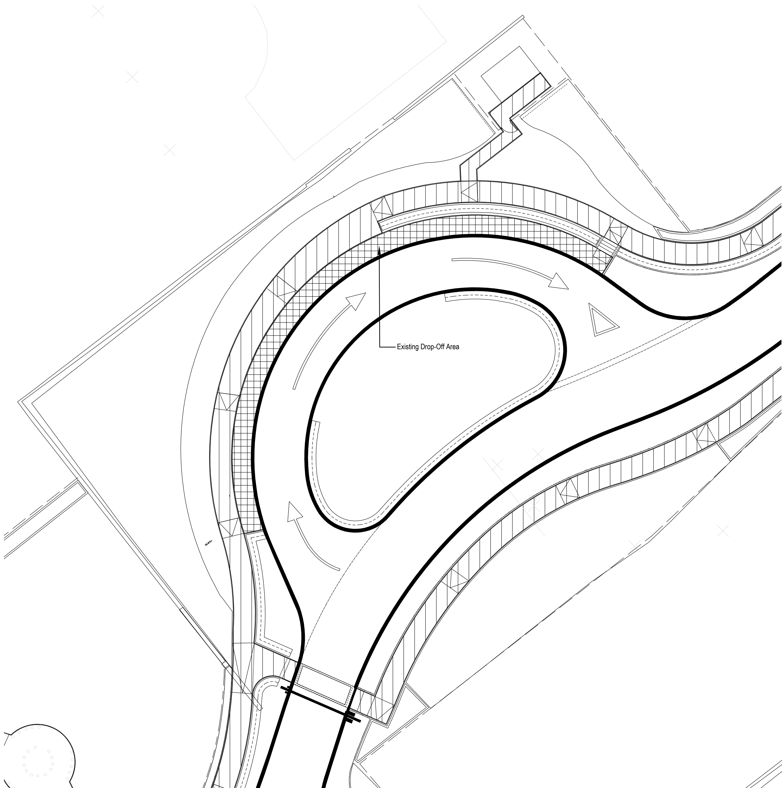
Existing Car Parking Layout
