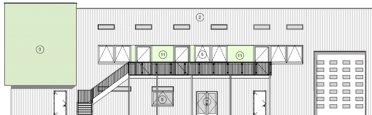
Proposed East Elevation 1:200 @ A3
