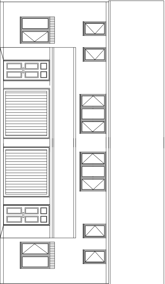
Front Elevation
