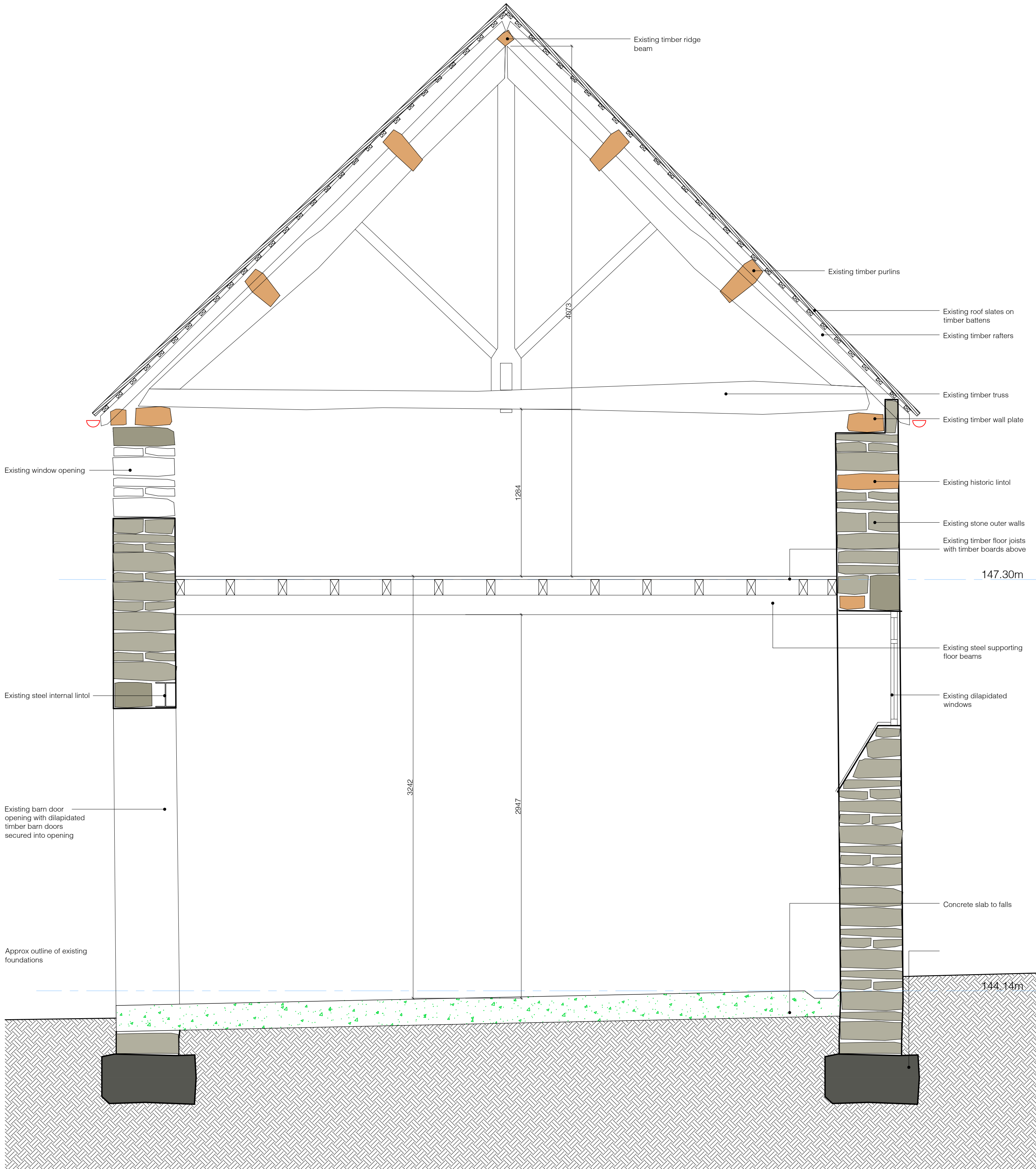
Barn 2 Existing section AA
