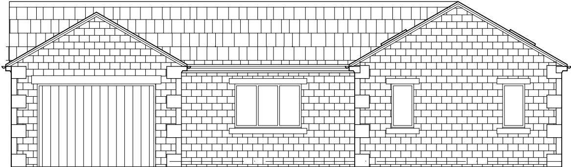
SIDE ELEVATION
