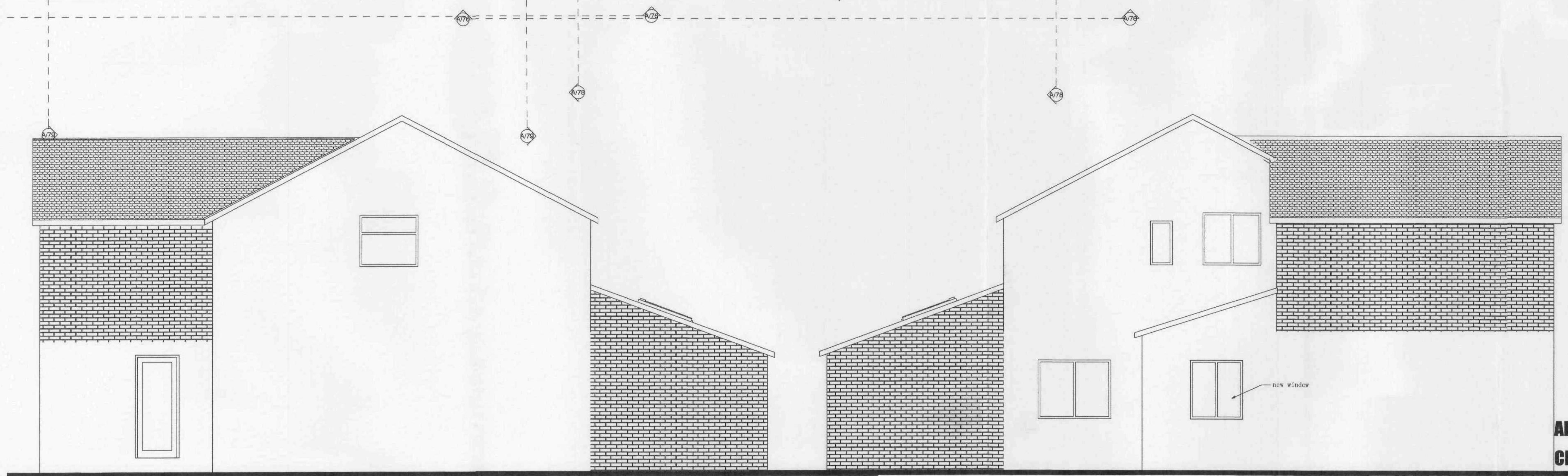
Elevation A/79
