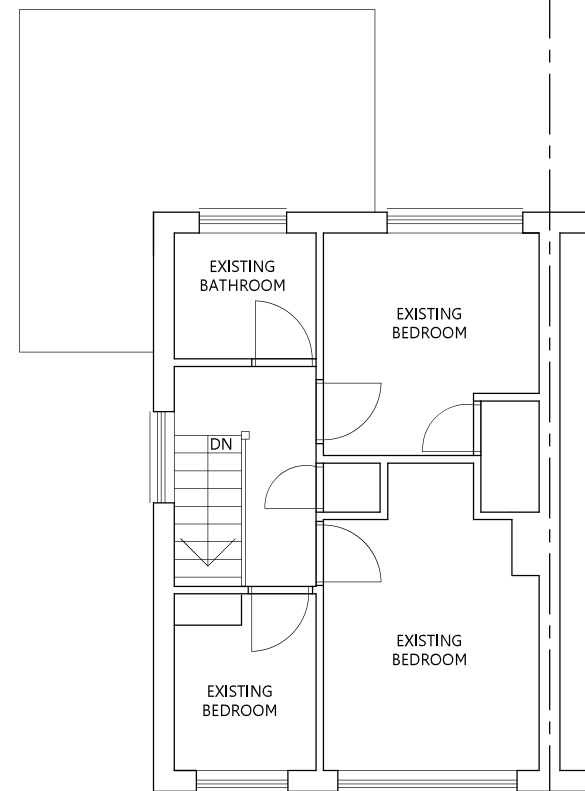
FIRST FLOOR PLAN 1:50
