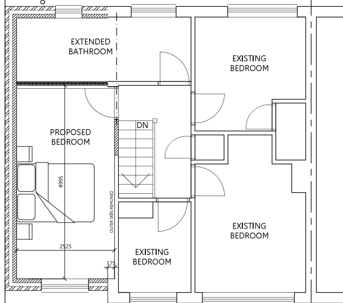
FIRST FLOOR PLAN 1:50
