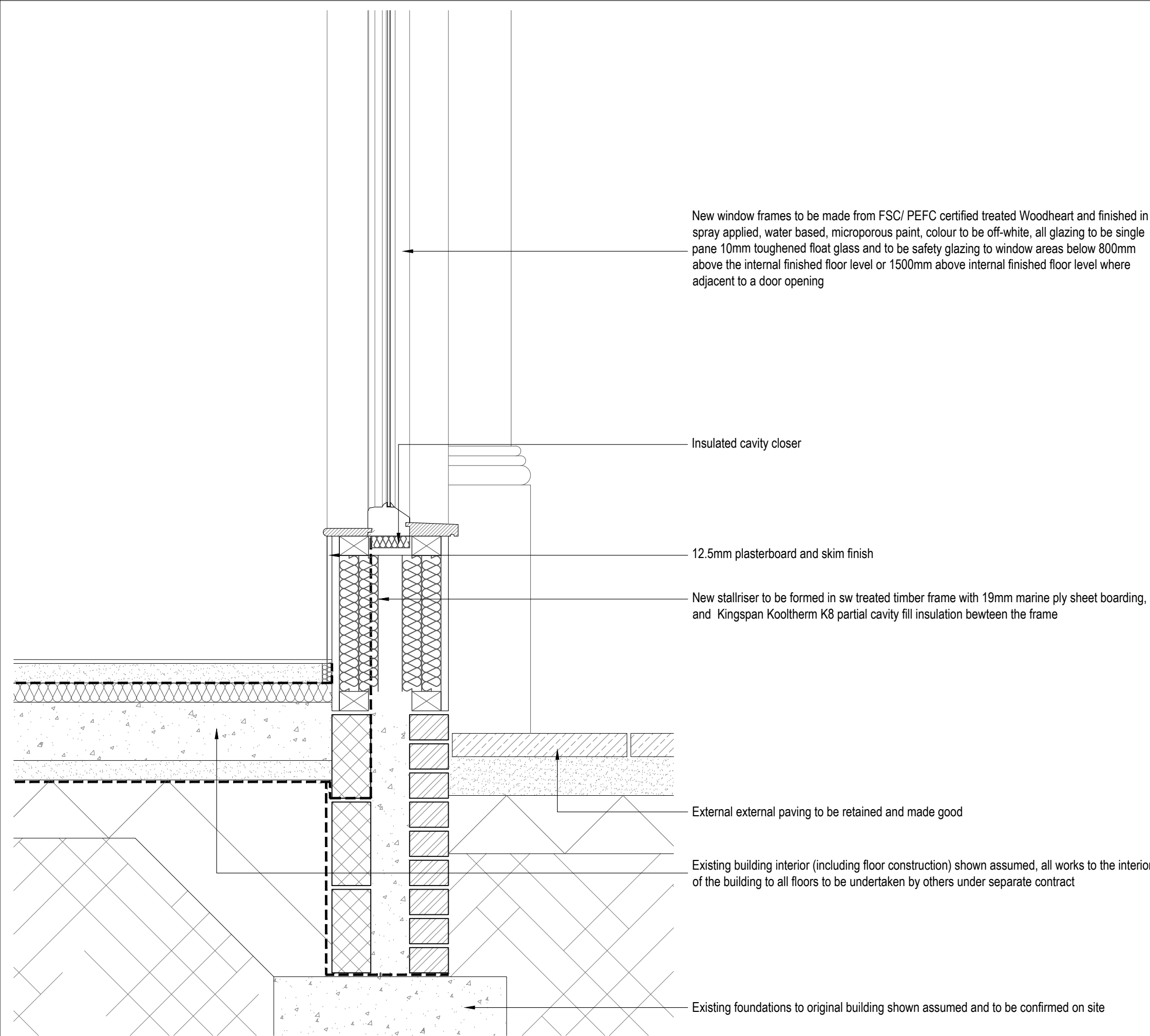
Typical Shop Frontage Stallriser Detail
