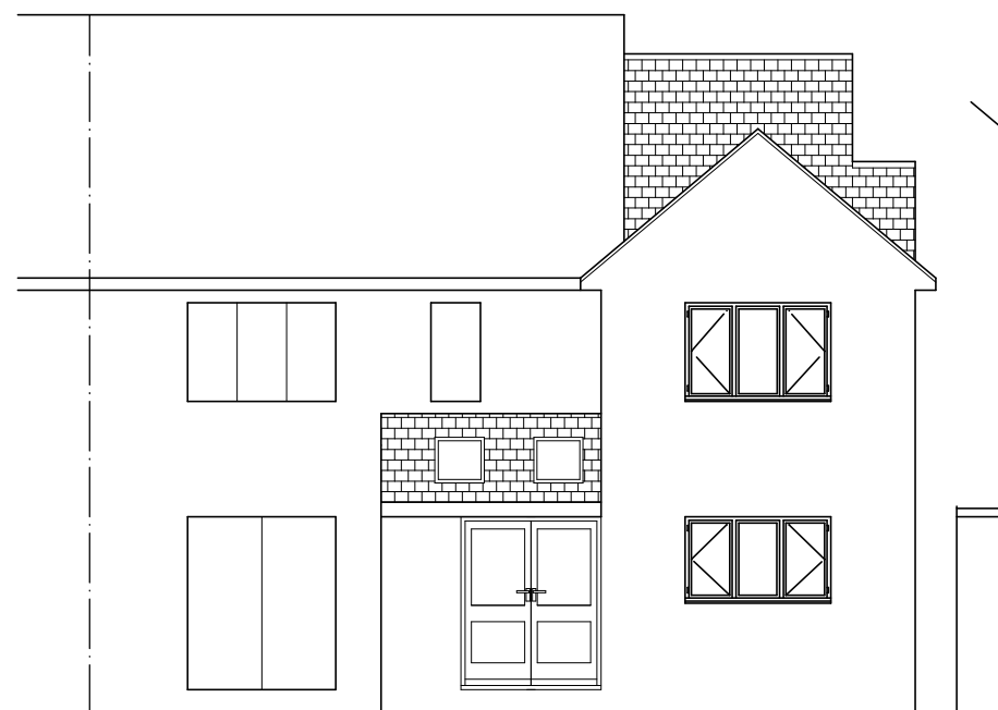
REAR ELEVATION
