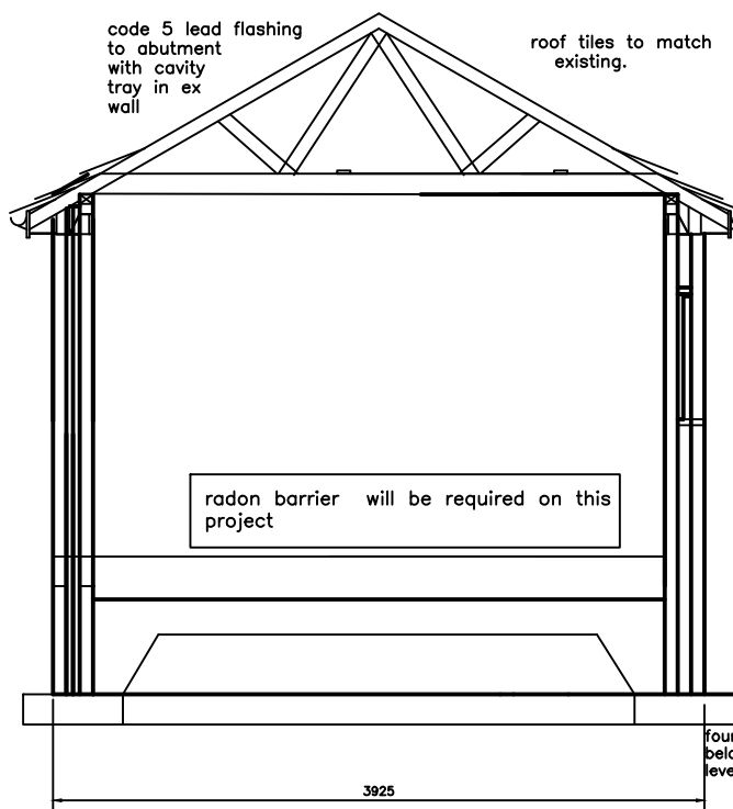
SECTION (typical)
