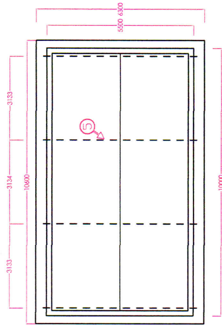
PLAN VIEW
