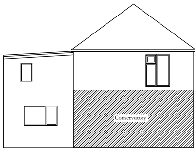
Rear Elevation 1:200
