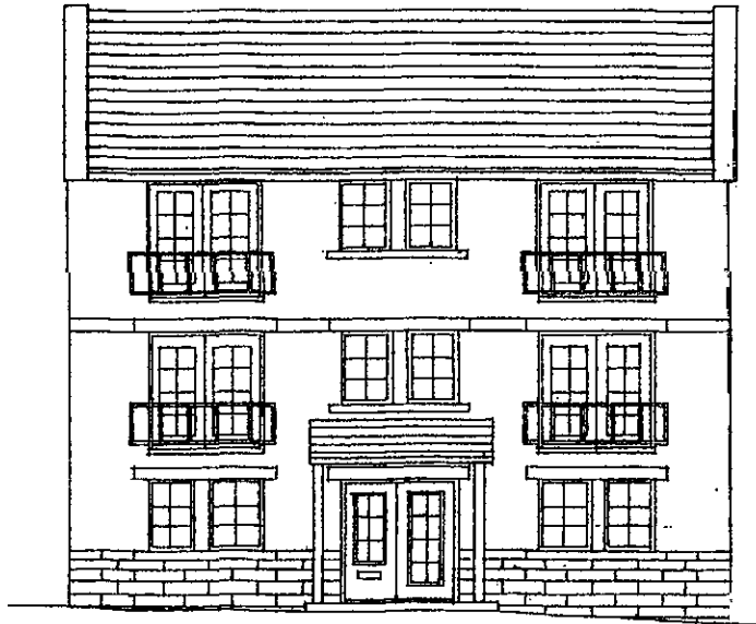
FRONT ELEVATION
