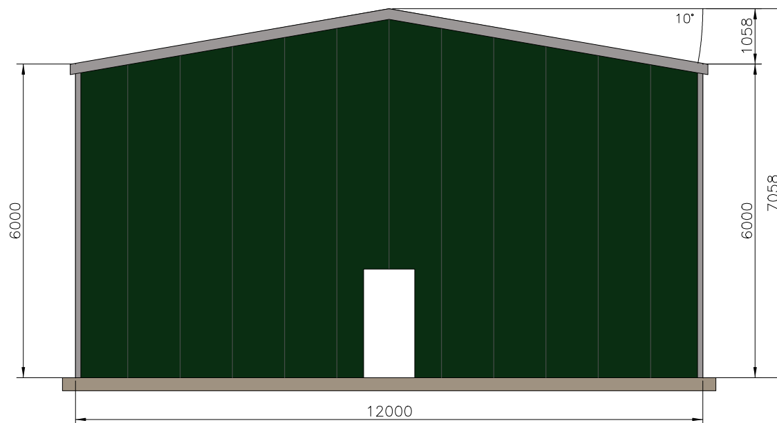
Front Elevation (External)
