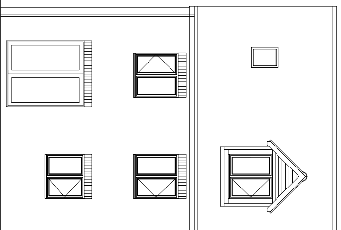
Rear Elevation
