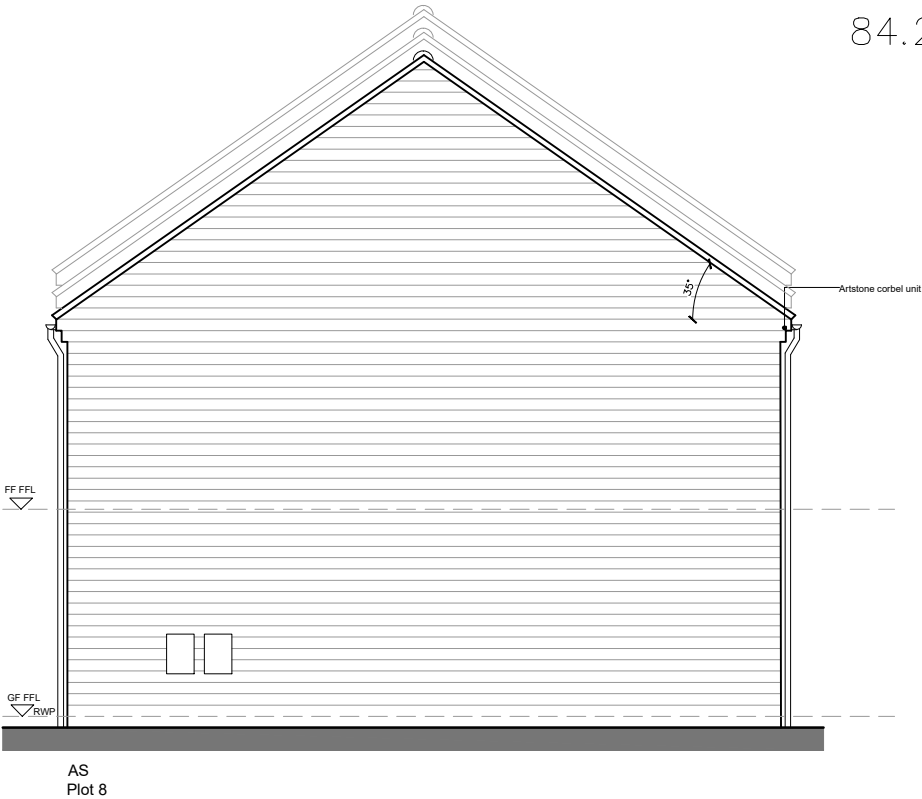
SIDE ELEVATION
