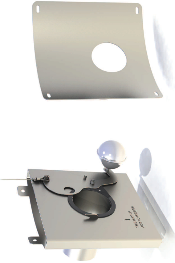
ACO Q-Plate with remote draindown and bypass recommended for all orifice apertures less than 100mm
