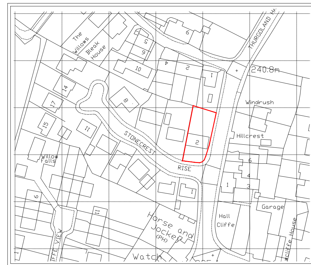
LOCATION PLAN 1:1250
