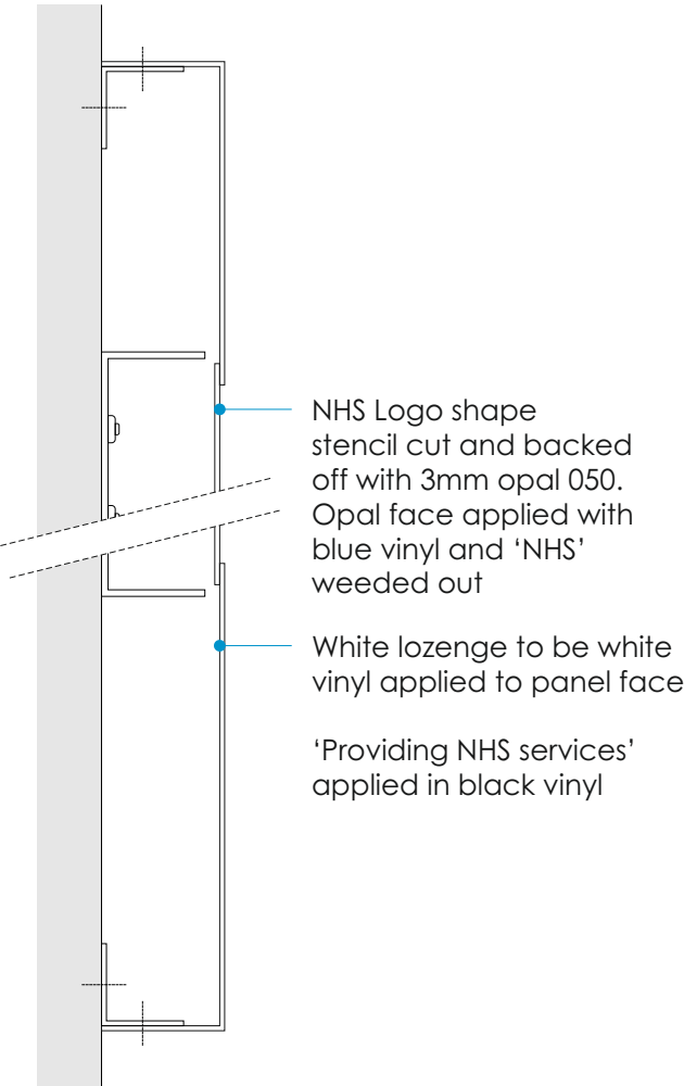
Section 1:5@A3
