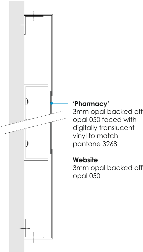
'Pharmacy' / website section 1:5@A3
