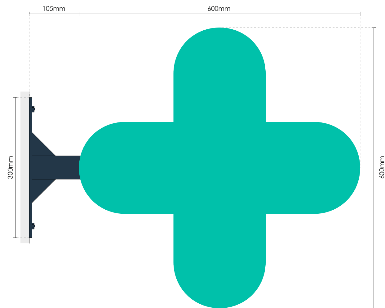
Face views Scale 1:5 @ A3
