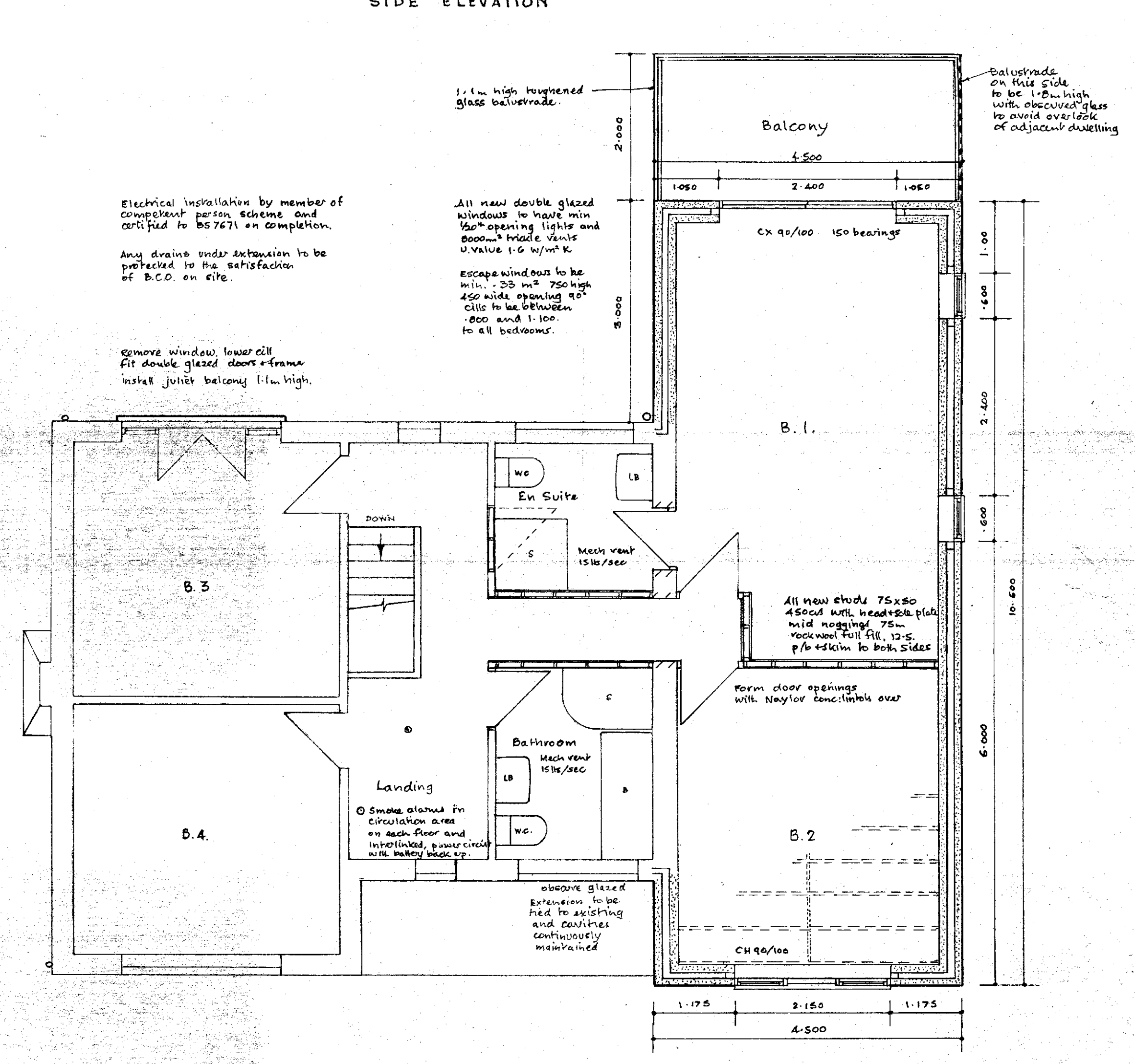
PROPOSED FIRST FLOOR
