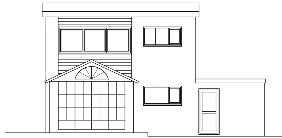
Existing Rear Elevation (West Facing)
