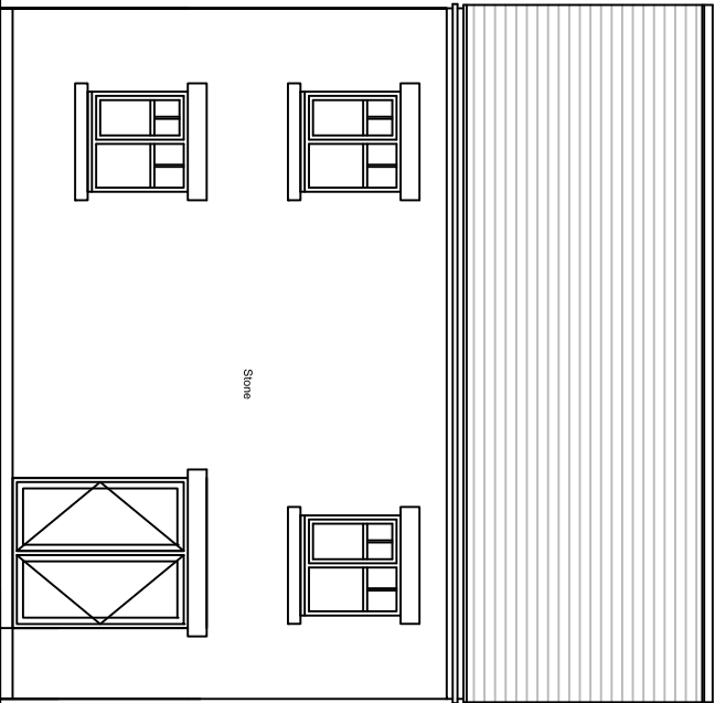
Rear Elevation 1:100
