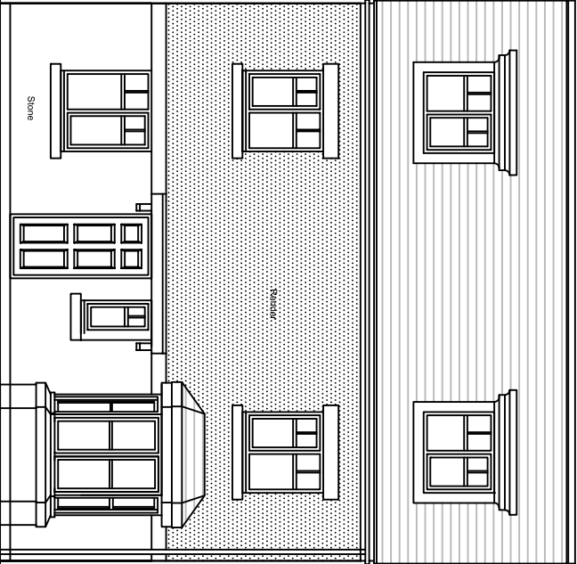
Front Elevation 1:100
