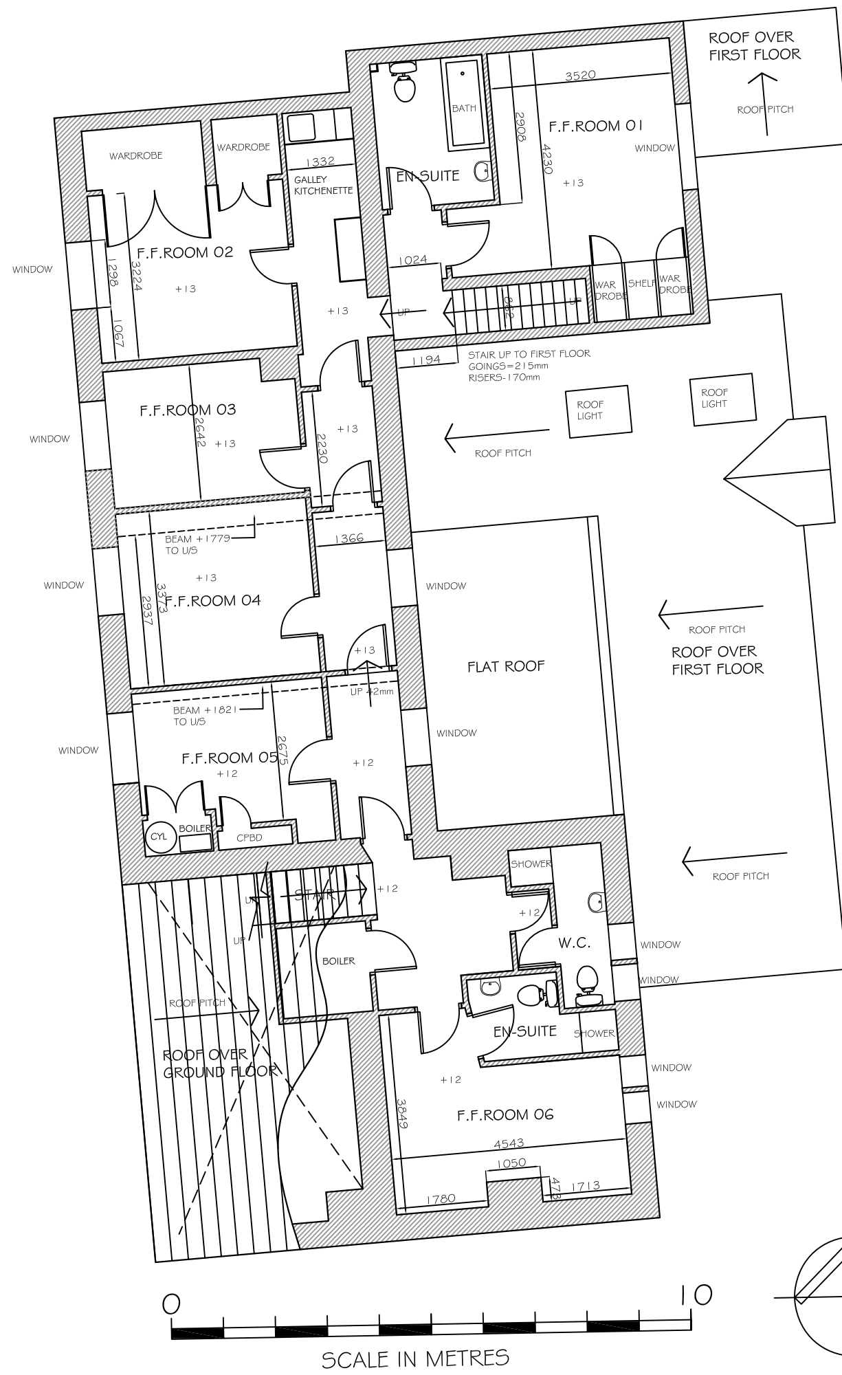
EXISTING FIRST FLOOR G.A.PLAN
