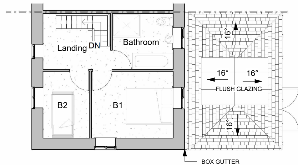
First Floor Plan 1 : 100
