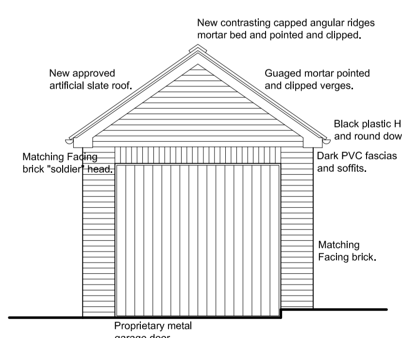
FRONT ELEV
