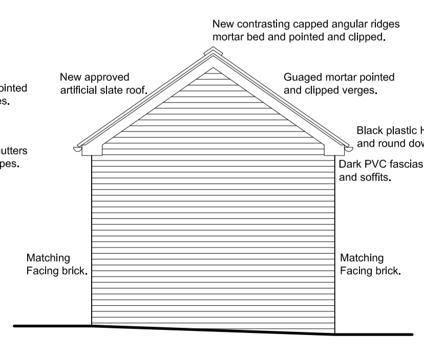
REAR ELEV
