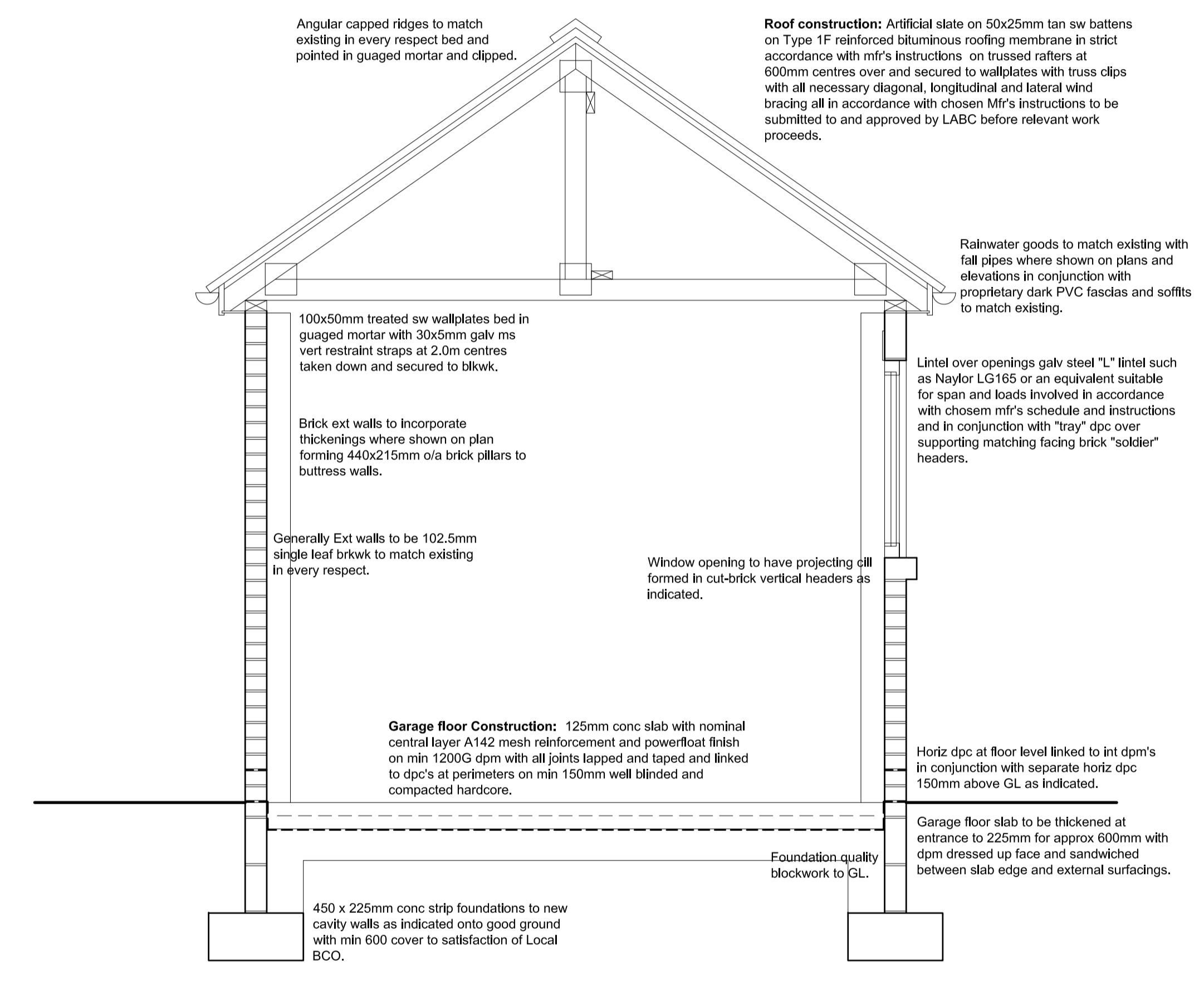
TYPICAL SECTION @ 1:20
