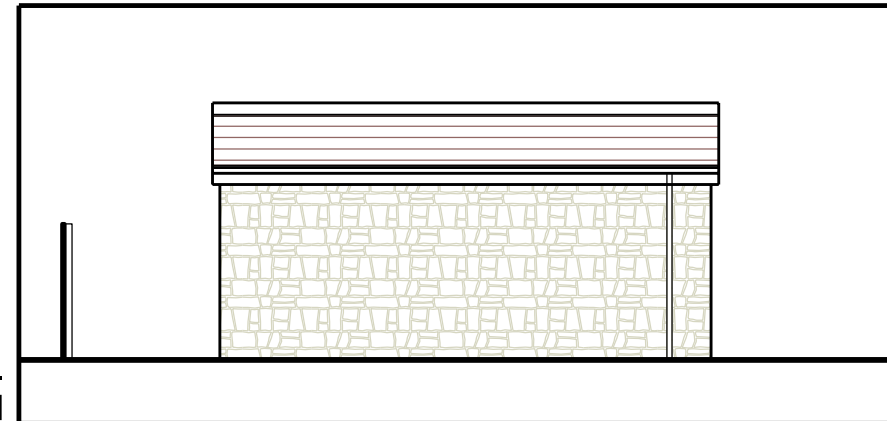
Garage North Elevation - Proposed
