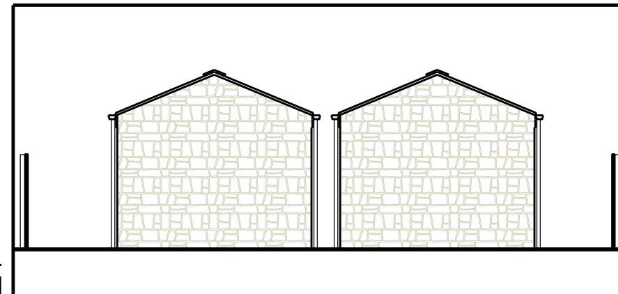
Garage East Elevation - Proposed
