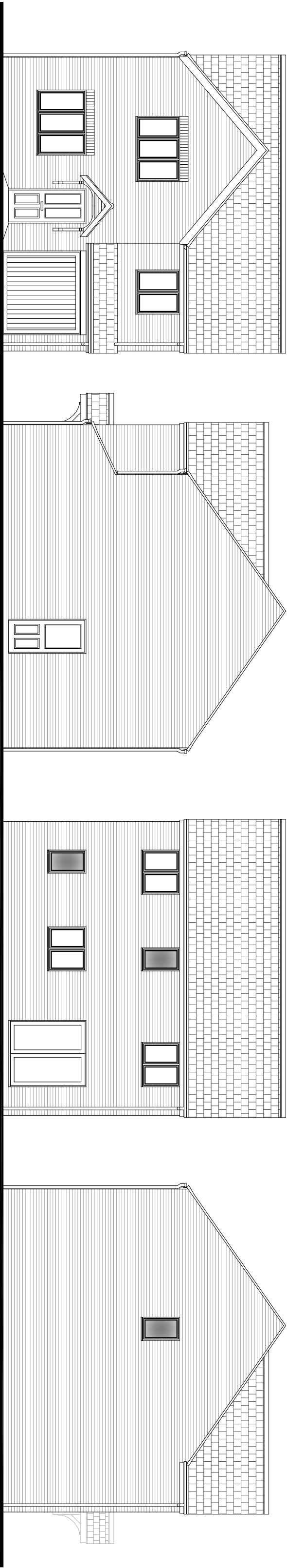
Front Elevation
