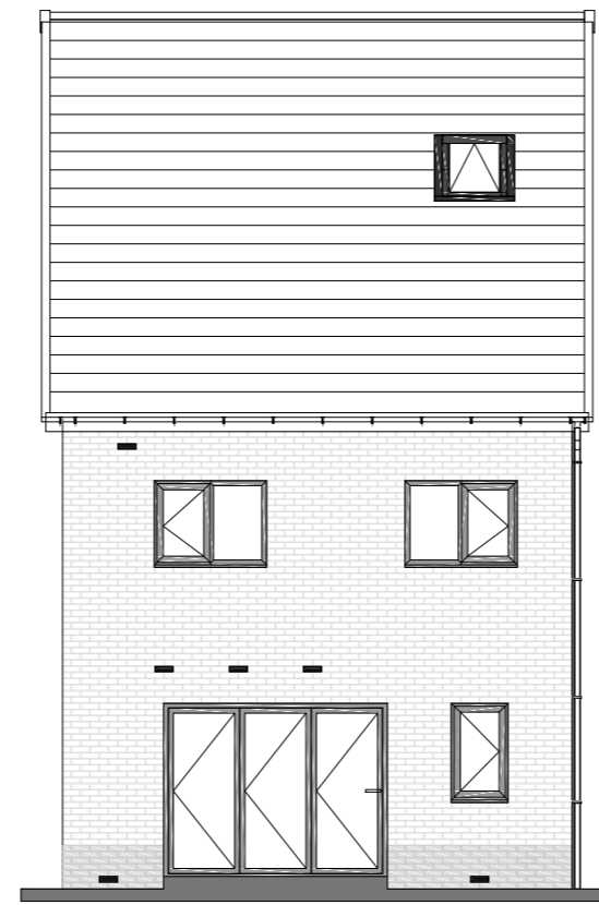
REAR ELEVATION
