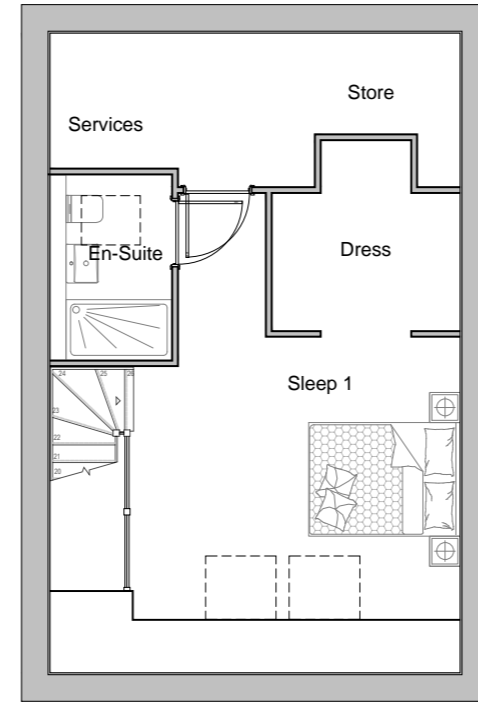
SECOND FLOOR
