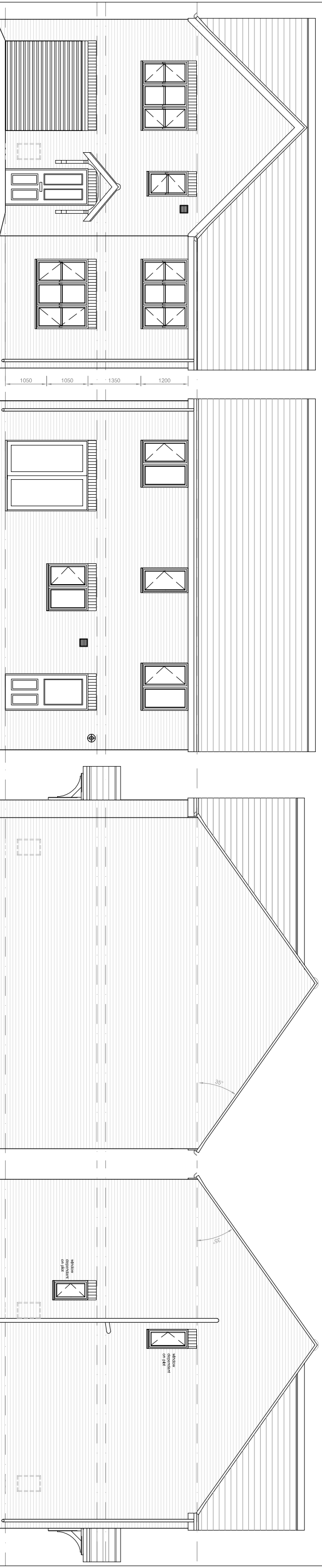
Front Elevation
