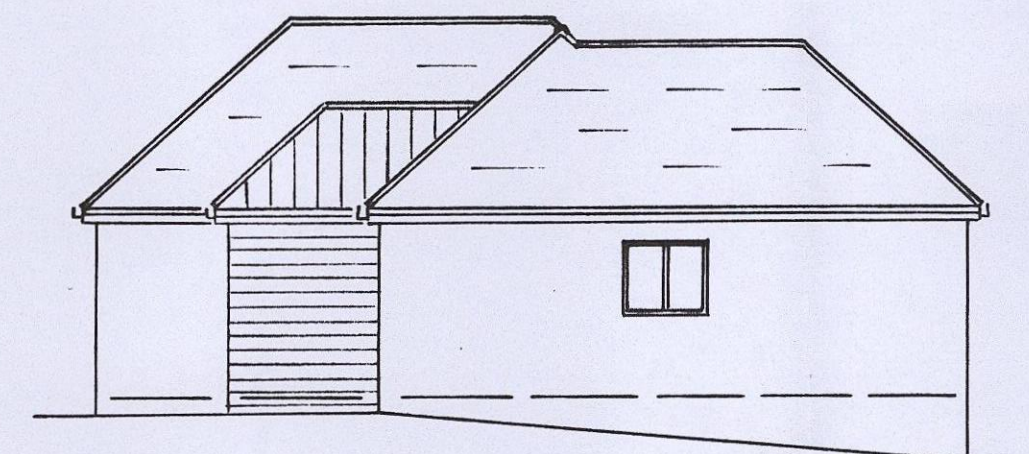
PROPOSED SIDE SOUTH - EAST
