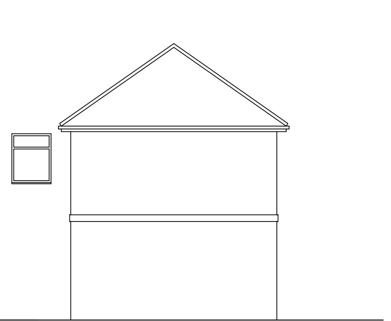
EX SIDE ELEVATION
