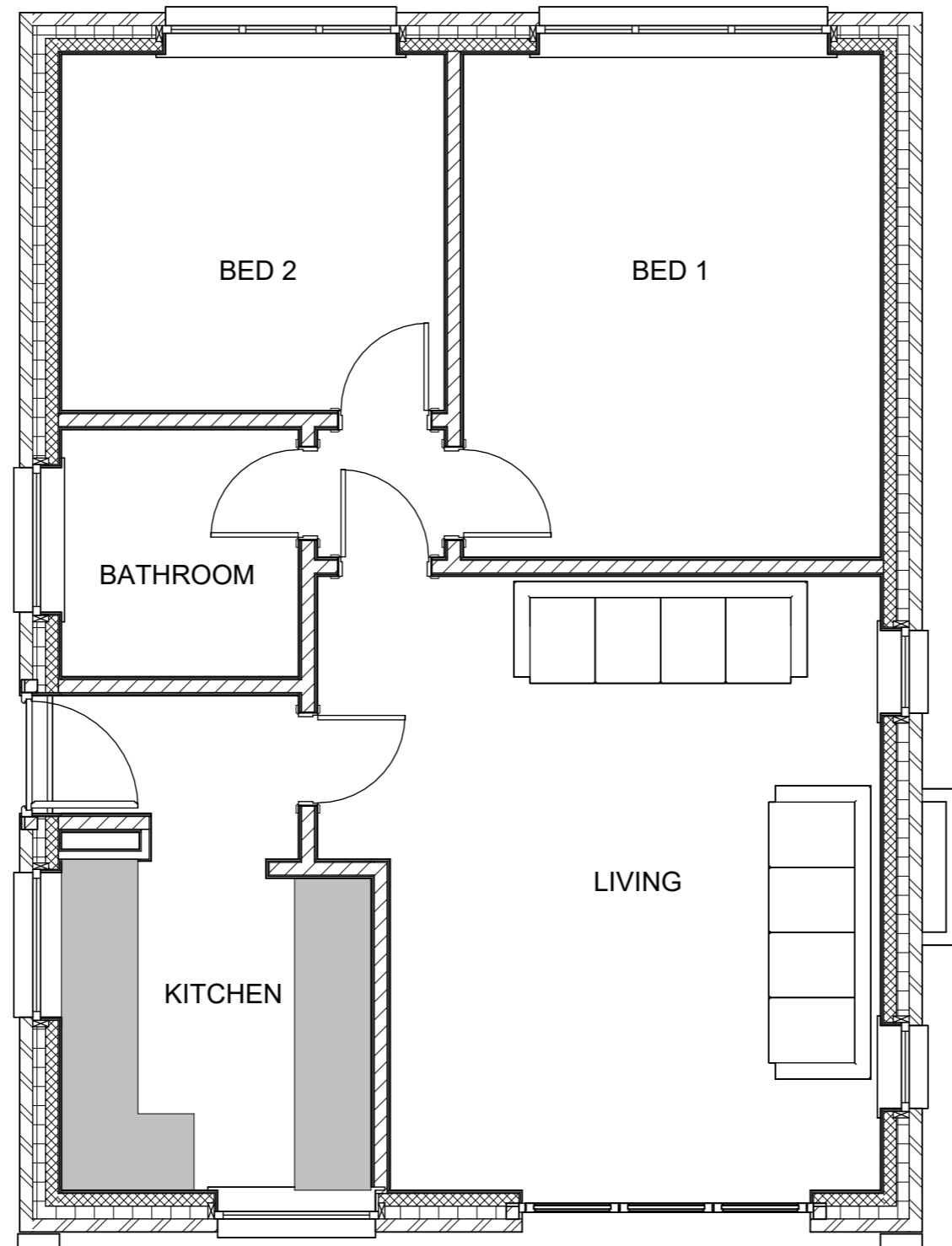
Existing GF Plan 1 : 50
