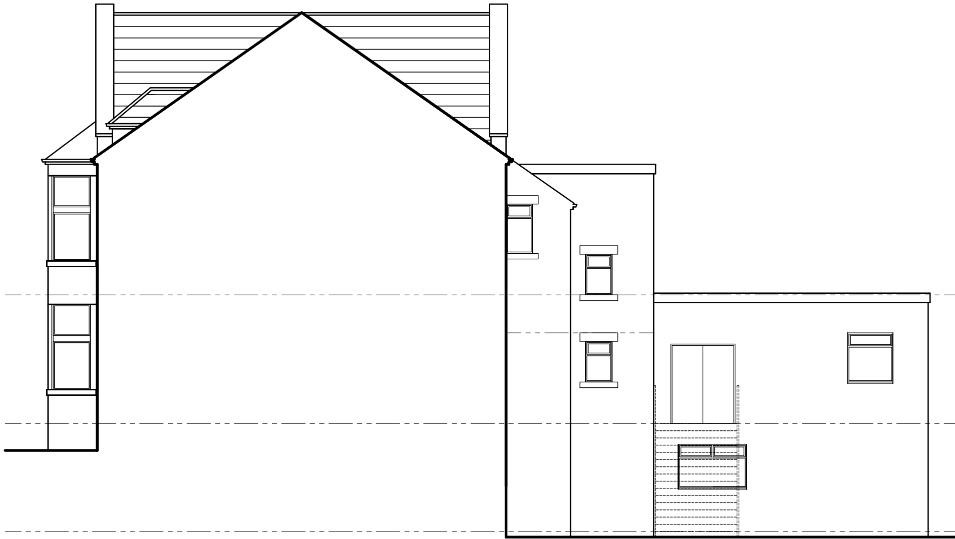
SIDE ELEVATION
