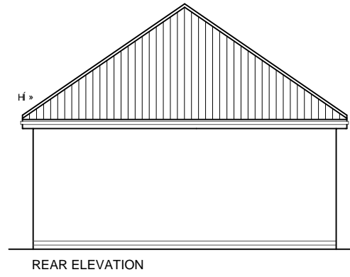
REAR ELEVATION
