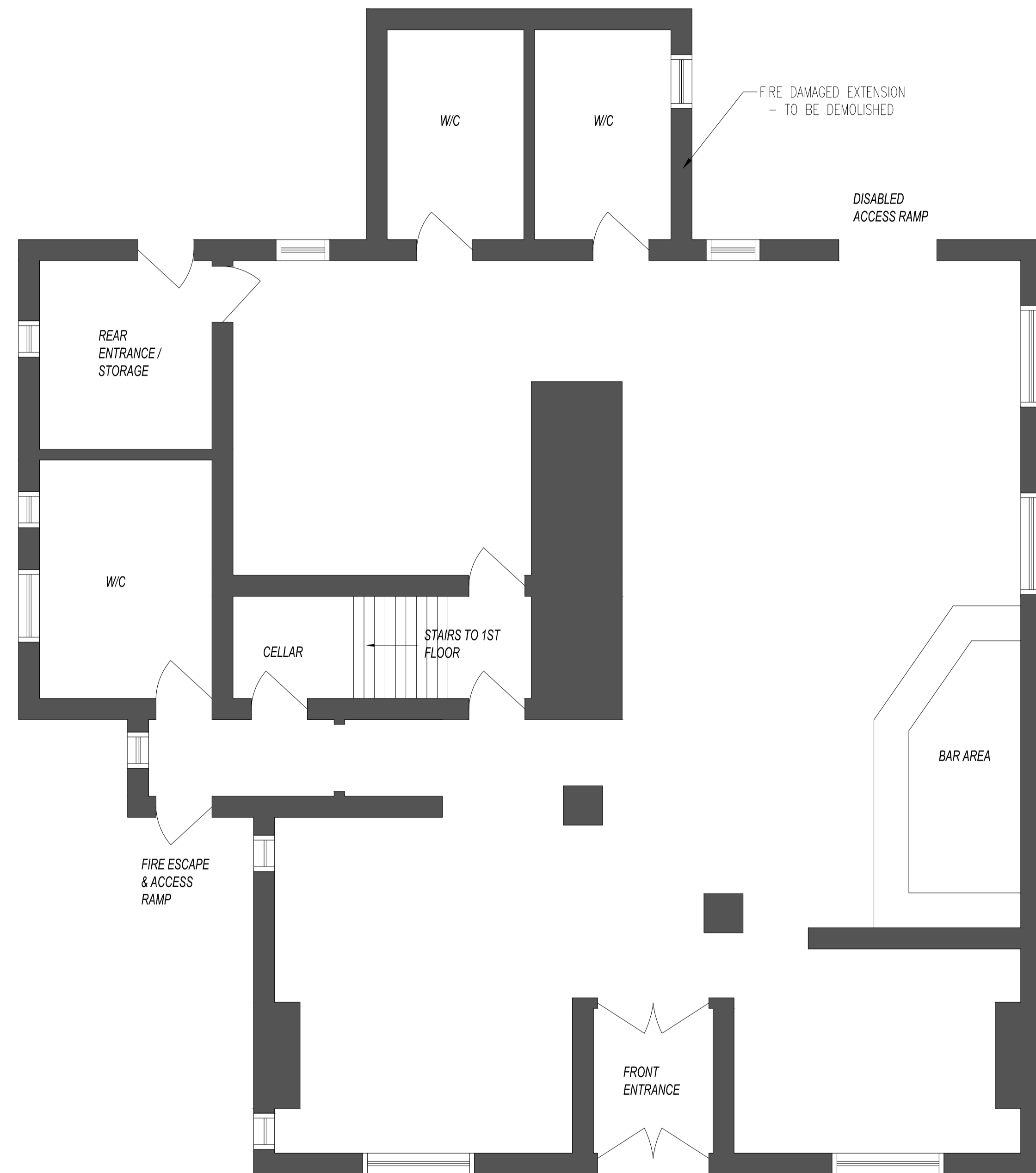
EXISTING GROUND FLOOR SCALE 1:50
