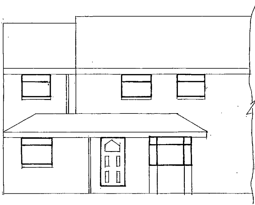
REVISED PROPOSED FRONT ELEVATION
