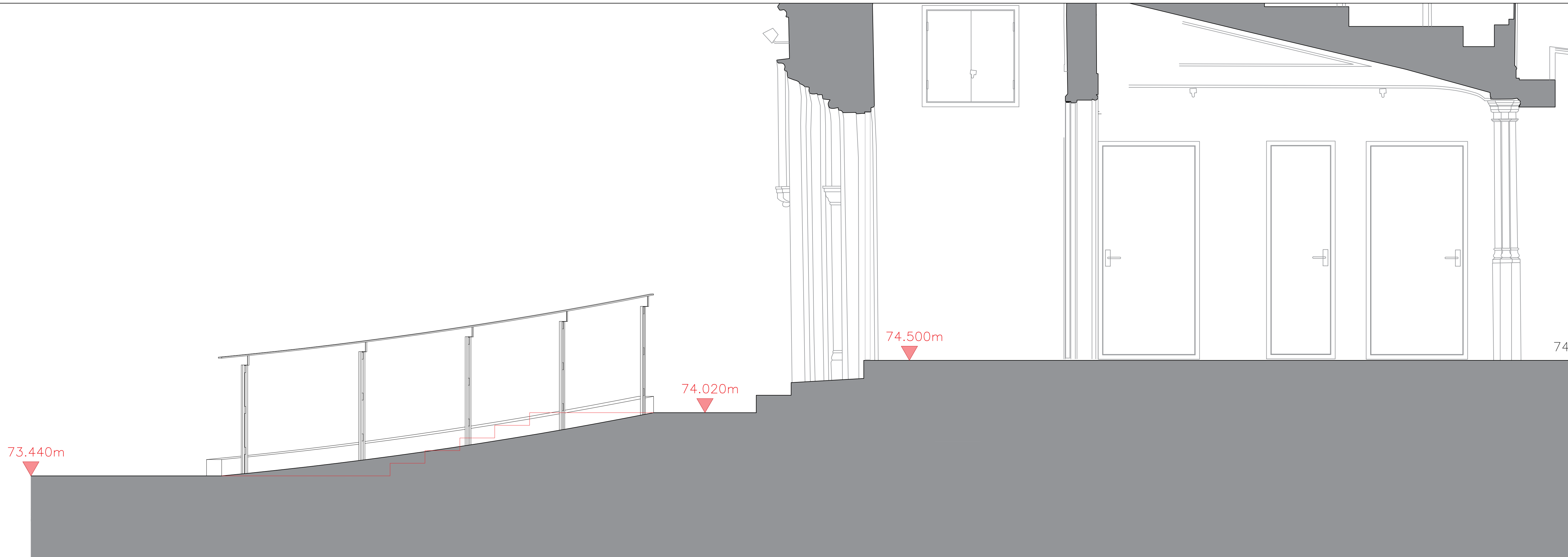
1 PROPOSED NARTHEX ENTRENCE SECTION WITH LEVELS Scale: 1:20
