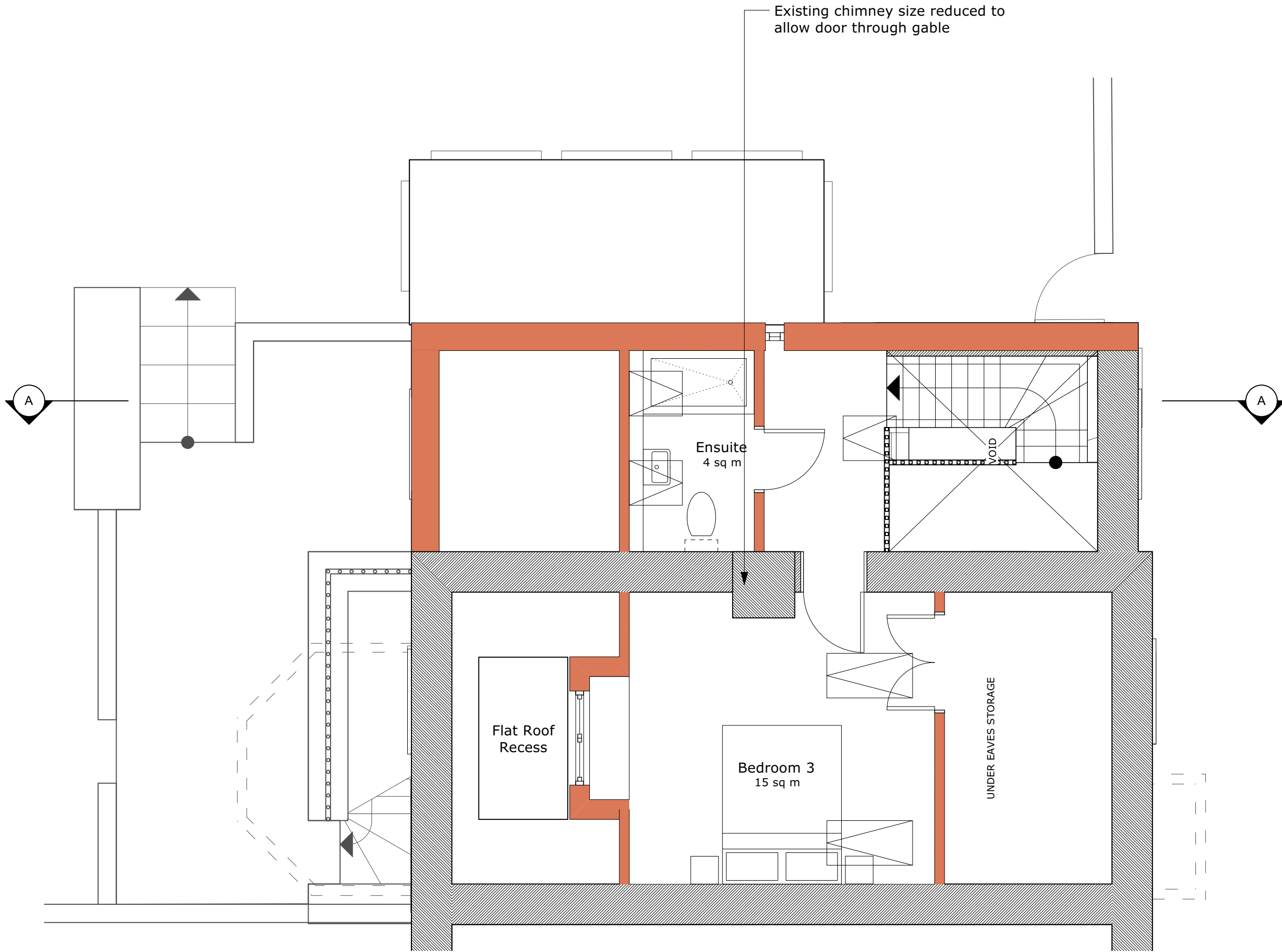
1 Proposed Second Floor Plan Scale: 1:50
