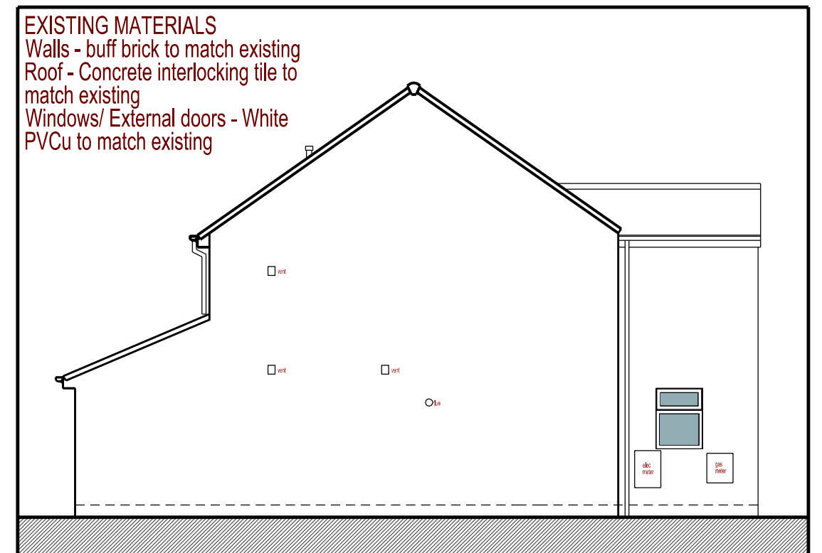
West Elevation - Proposed
