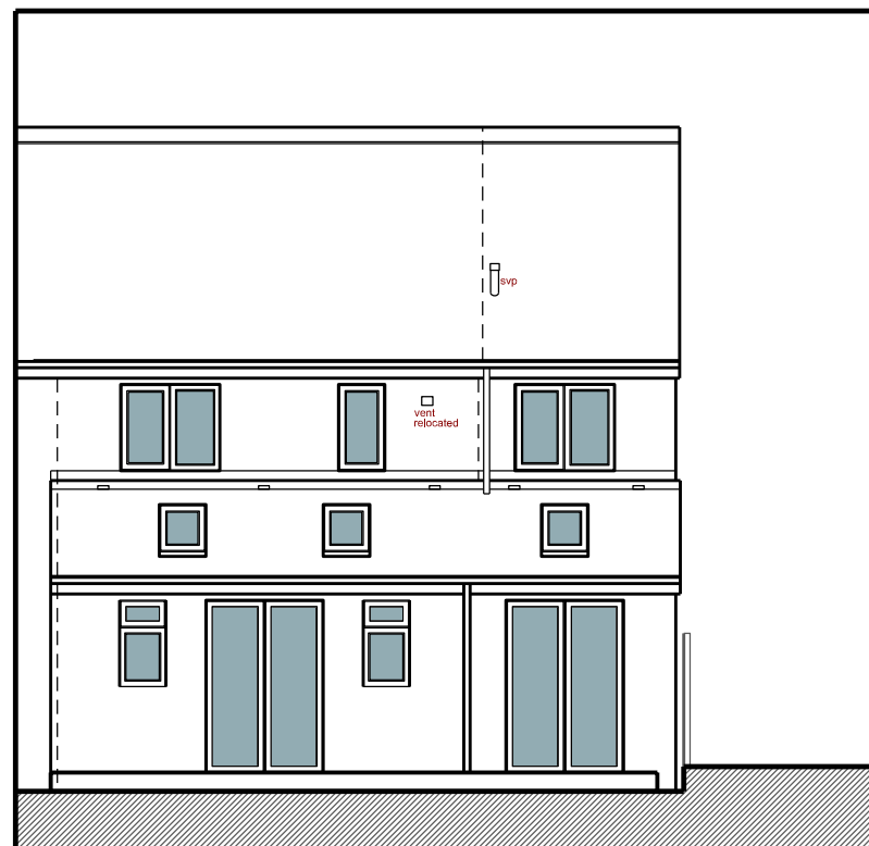
North Elevation - Proposed
