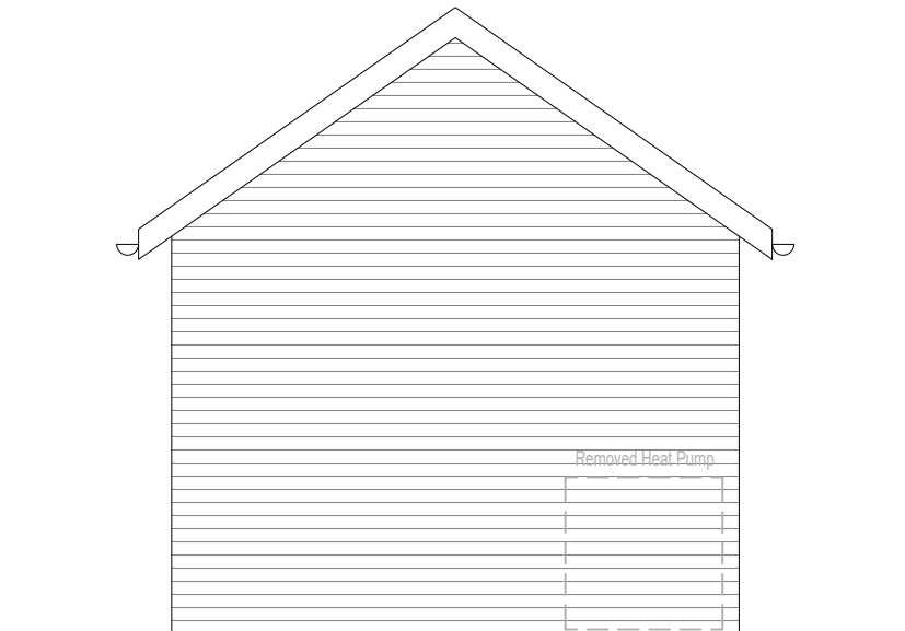
NORTH-WEST ELEVATION
