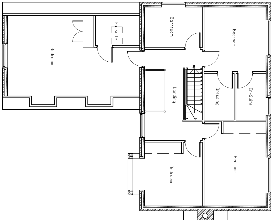
First Floor
