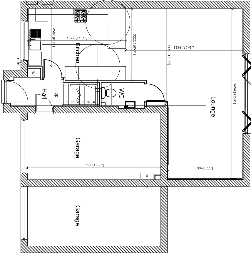
HOUSE TYPE A GROUND FLOOR PLAN
