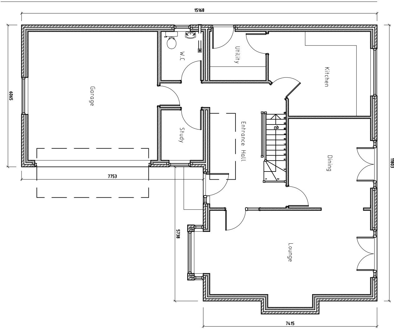
Ground Floor
