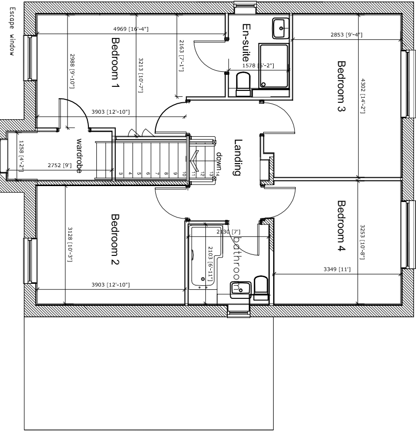
HOUSE TYPE A FIRST FLOOR PLAN
