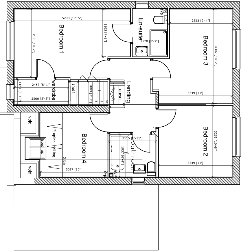
HOUSE TYPE B FIRST FLOOR PLAN
