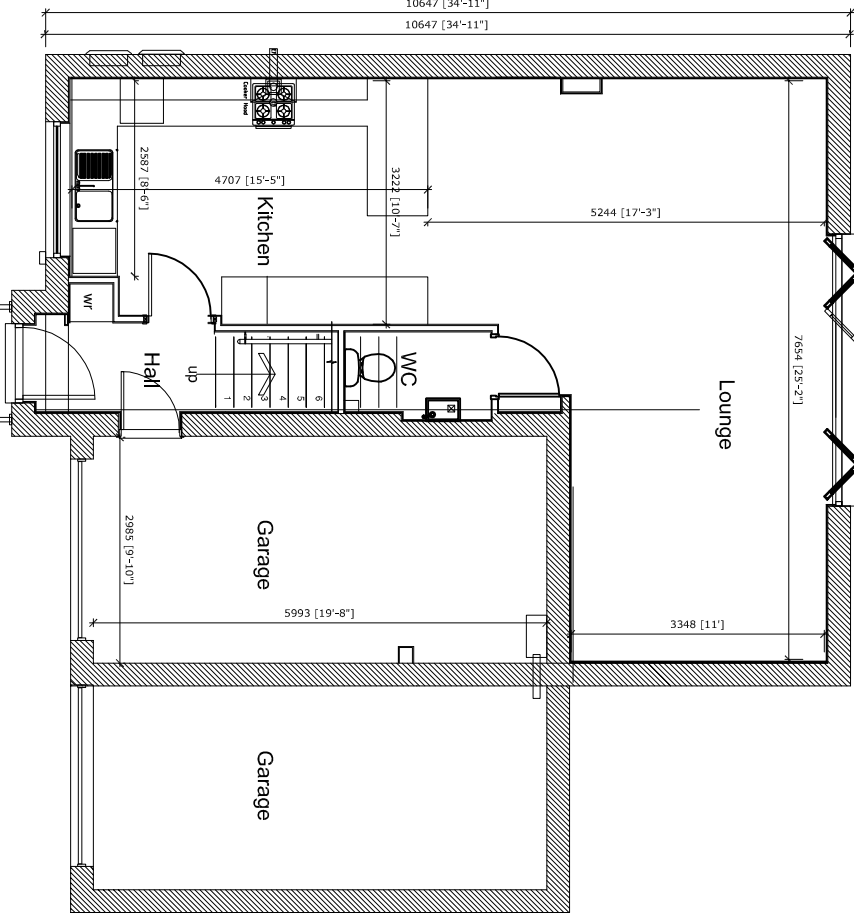
HOUSE TYPE B GROUND FLOOR PLAN
