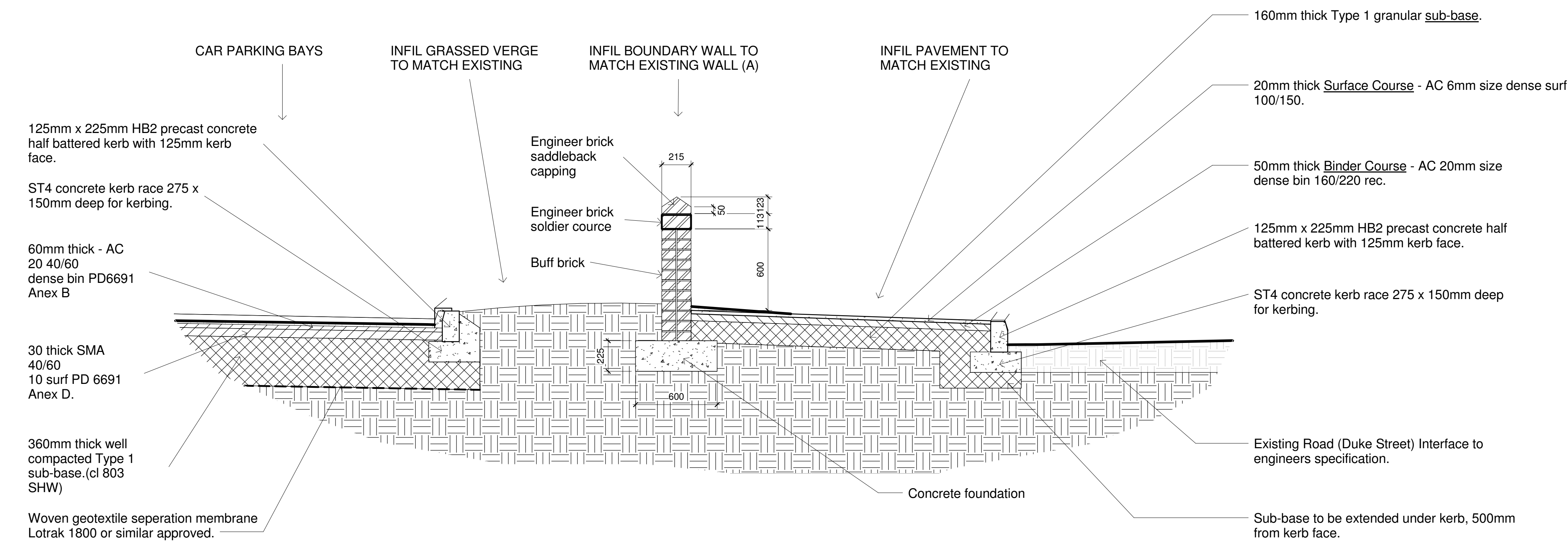
2 Section Duke Street Infil Boundary Wall - Detail 1 : 20
