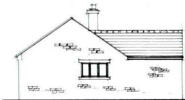
SIDE ELEVATION - NORTH
