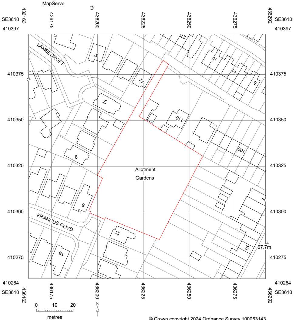
1 Location Plan 1 : 1250
