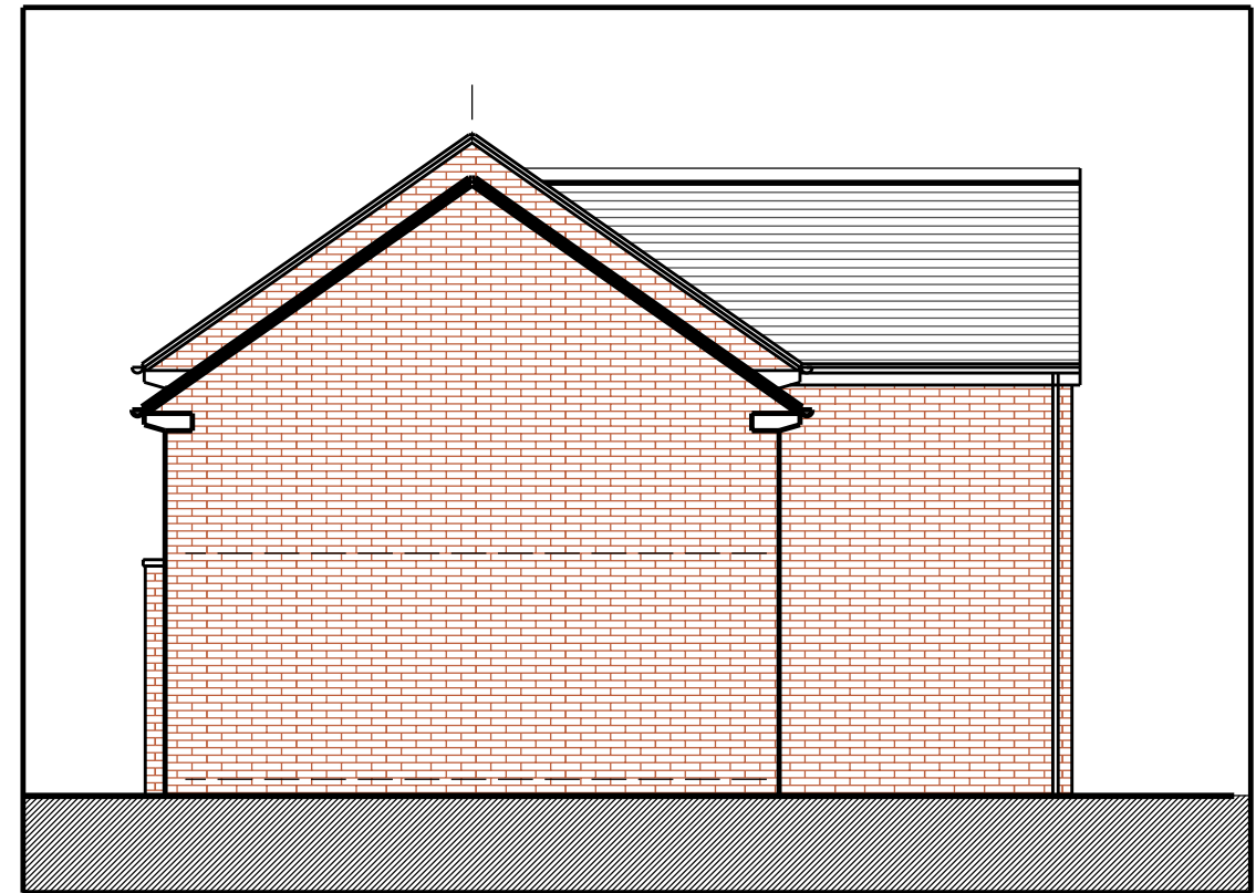
East Elevation
