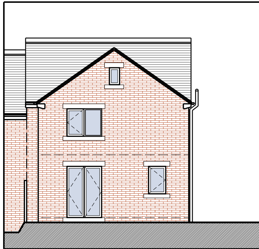
North Elevation
