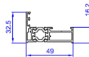
APE 3025 OUTER FRAME
