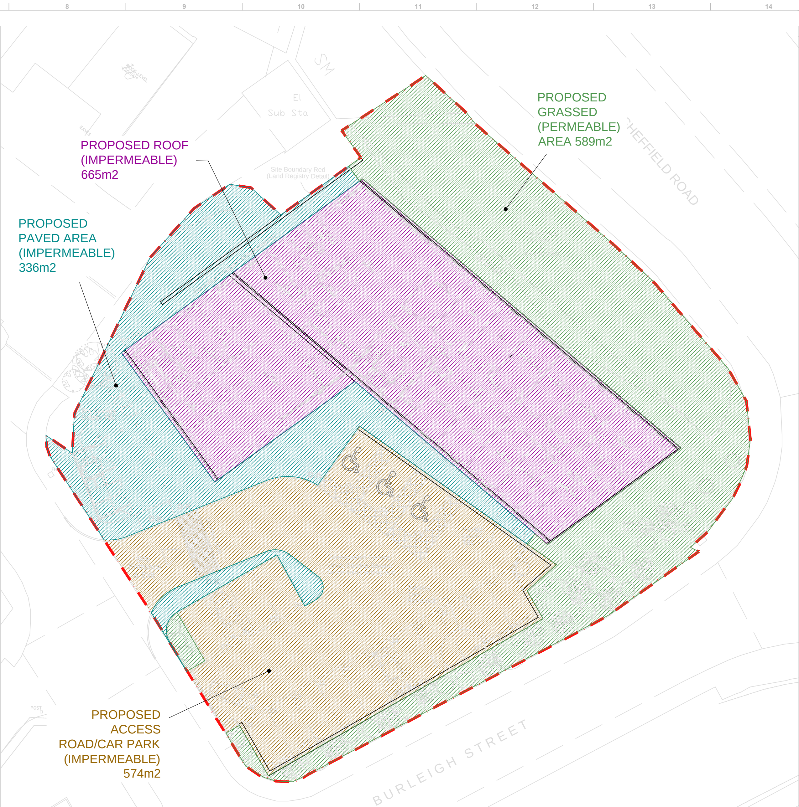
IMPERMEABLE/PERMEABLE AREAS (PROPOSED) SCALE 1:200 TOTAL PROPOSED IMPERMEABLE AREA = 1575 m2 TOTAL PROPOSED PERMEABLE AREA = 589 m2 2164 m2
