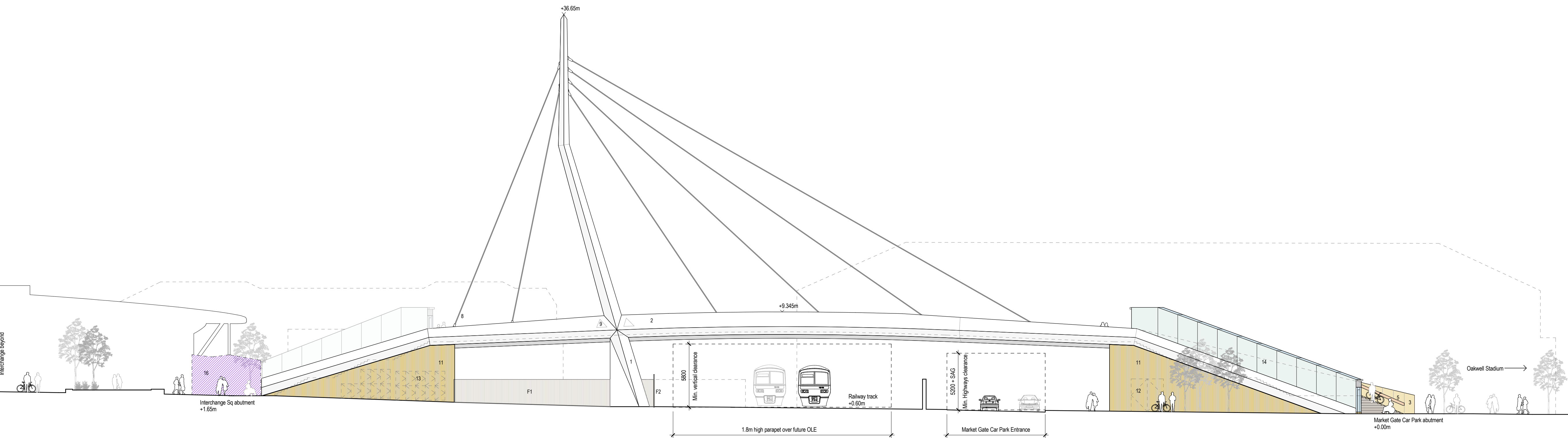
Proposed Elevation A (North) 1:200
