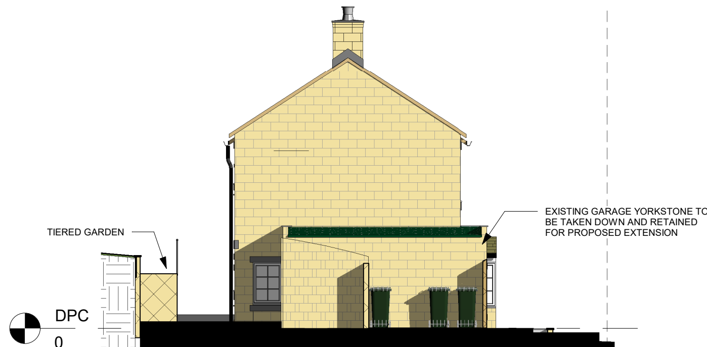
Left Elevation 1 : 100
