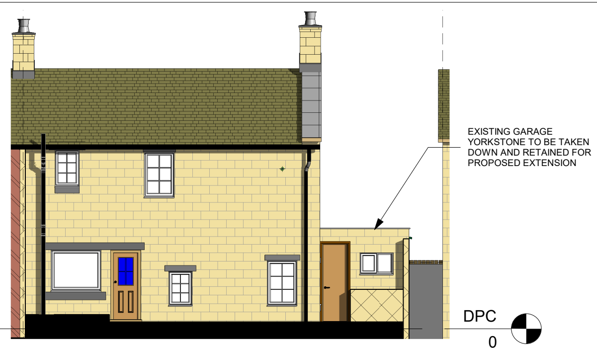
Rear Elevation 1 : 100
